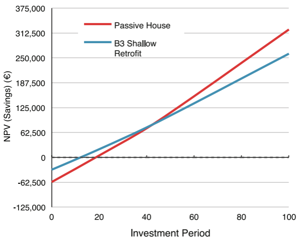
Figure 3. Sensitivity analysis: effect of varying discount rate, fuel inflation rate and investment period on NPV (cost savings).
